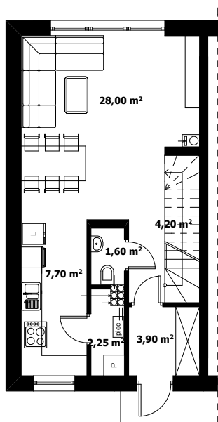
PARTER
