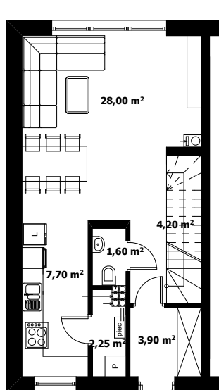
PARTER
